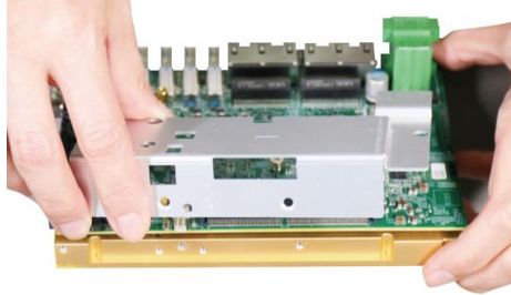
Install heatsink
