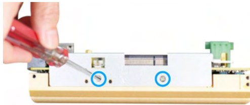
Remove the screws securing heat spreader
